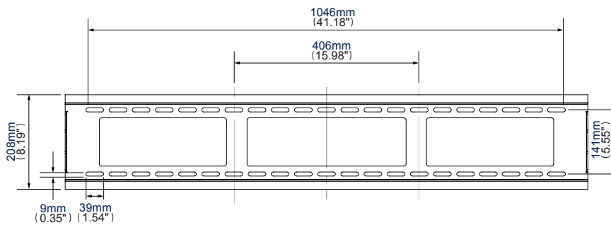
Wall Plate
